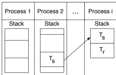
Fig. 2. KAAPI processor model.
