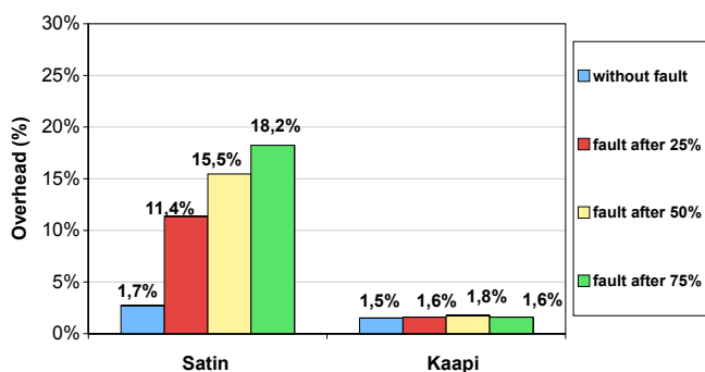
Fig. 13. Comparison of Satin with KA-API/ TIC using 32 Processors.
