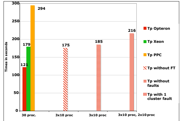
Fig. 12. QAP Application on Grid5000.
