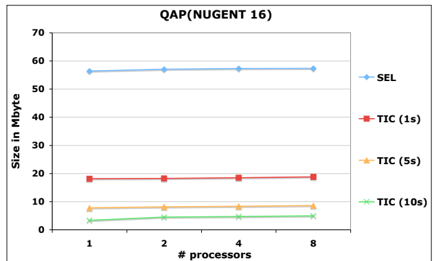
Fig. 9. Total Volume of Data Stored.
