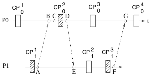
Fig. 5. TIC protocol: local and forced checkpoints.
