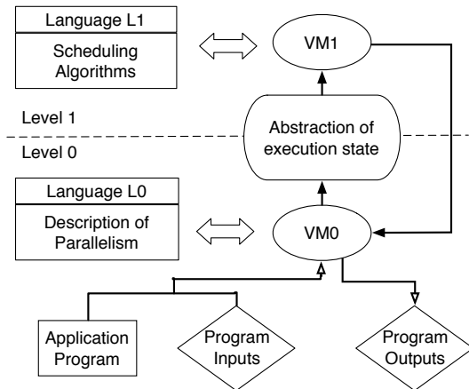
Fig. 1. Execution Model
