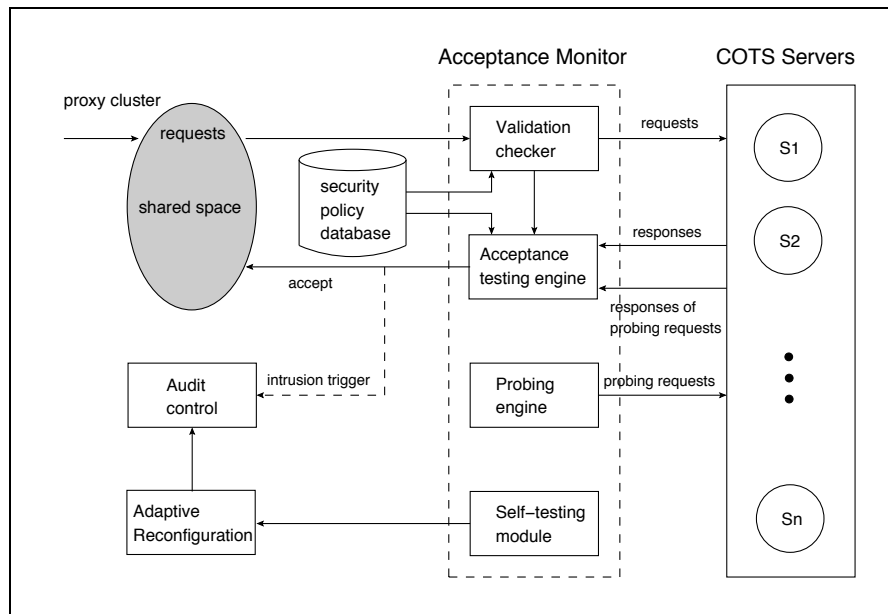
Fig. 4. Architecture of Acceptance Monitor
