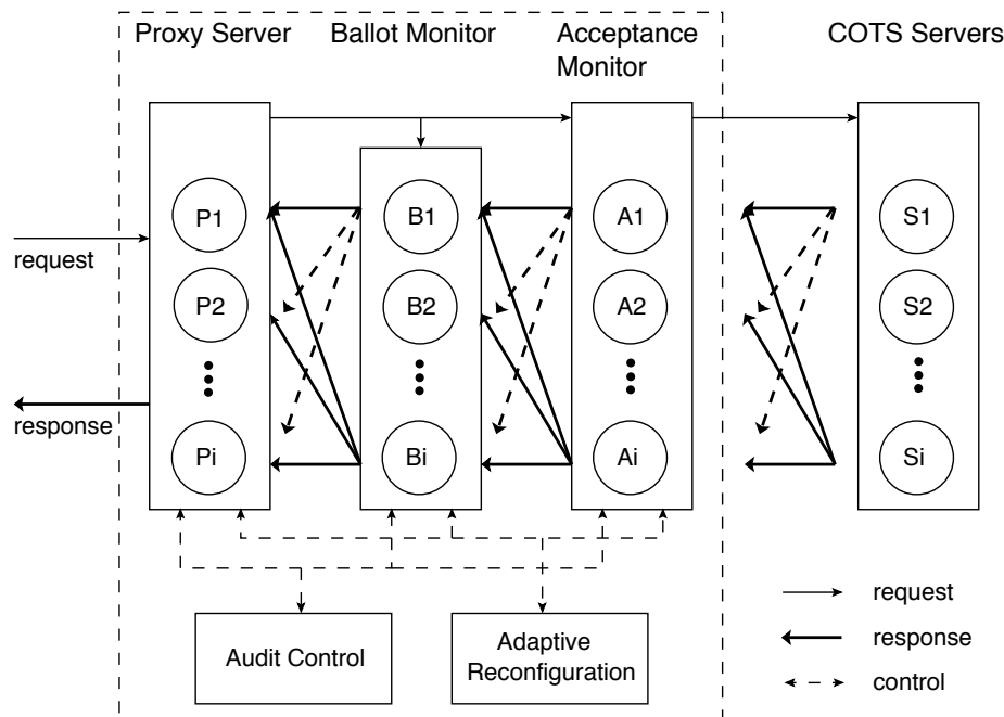
Fig. 1 generic intrusion- tolerant service architecture
