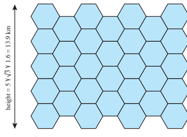
(a) Cell radius = 1.6 km
