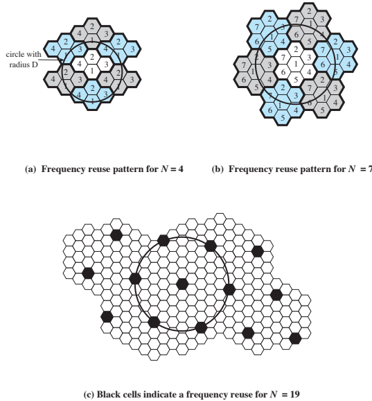
Figure 10.2 Frequency Reuse Patterns
