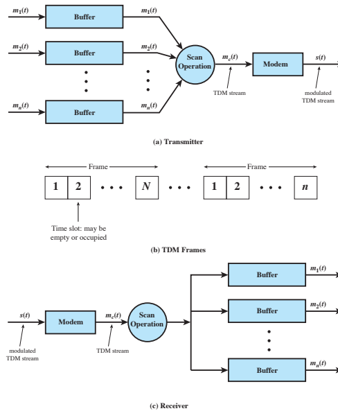
Figure 8.6 Synchronous TDM System
