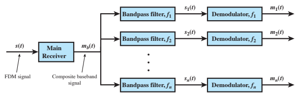
(c) Receiver
