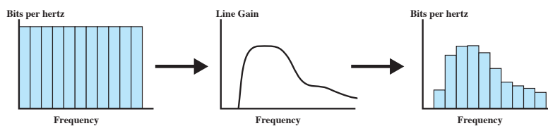
Figure 8.15 DMT Bits per Channel Allocation
