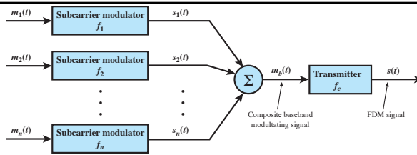
(a) Transmitter
