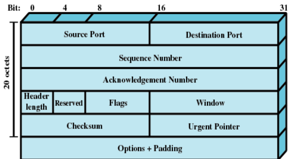
(a) TCP Header
