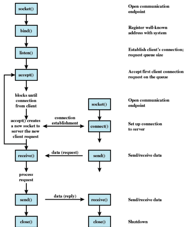
Figure 13.6 Socket System Calls for Connection-Oriented Protocol
