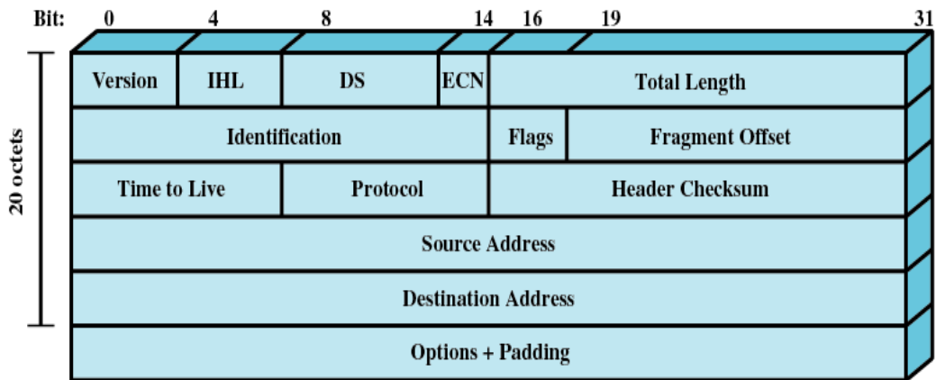
(a) IPv4 Header
