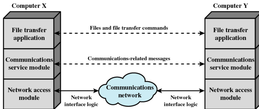
Figure 13.1 A Simplified Architecture for File Transfer
