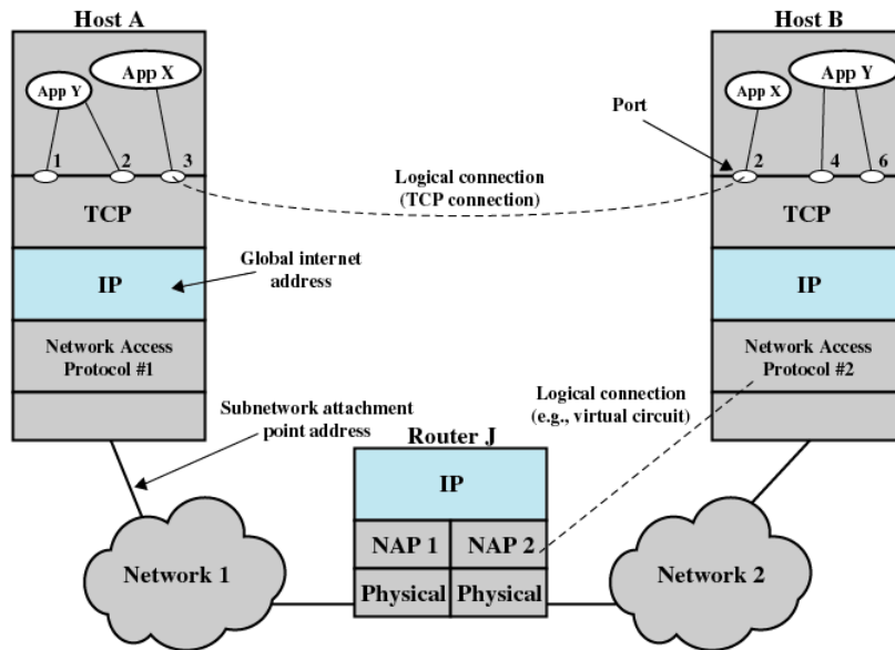
Figure 13.4 TCP/IP Concepts
